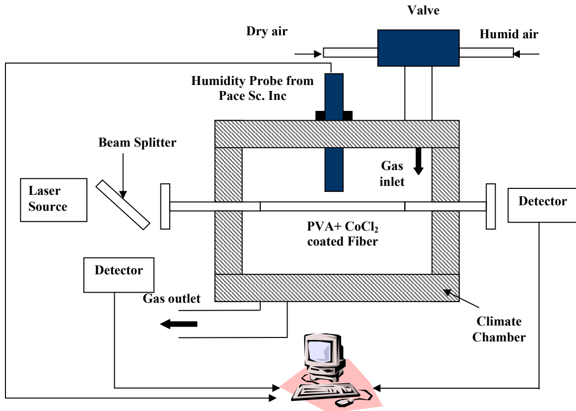
Figure 3.3 Experimental set-up
